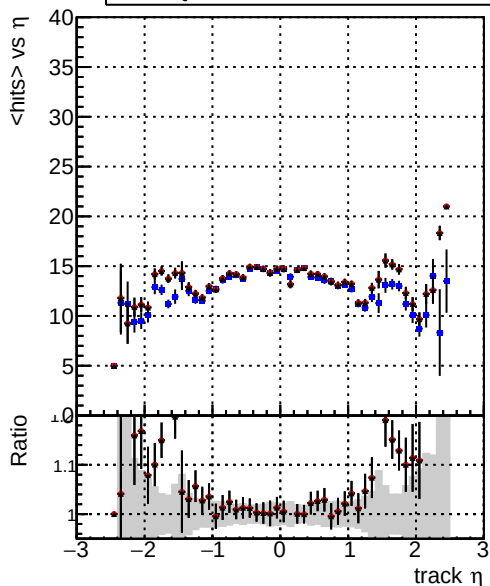
mean hit — DQM_CKF_TTbar — DQM_mkFit_TTbarPU-ncp — DQM_mkFit_TTbarPU-newTr5
