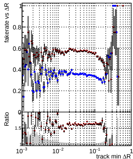
Legend: DQM_CKF_TTbar (blue circles) DQM_mkFit_TTbarPU-ncp (red circles) DQM_mkFit_TTbarPU-newTr5 (black circles)
