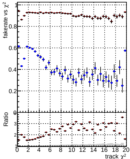
Fake rate vs. DOM CKF TTbar DOM mktFit TTbarPU-ncp DOM mktFit TTbarPU-newTr5
