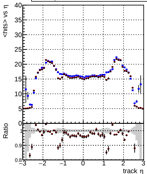
mean hit — DQM_CKF_TTbar — DQM_mkFit_TTbarPU-ncp — DQM_mkFit_TTbarPU-newTr5
