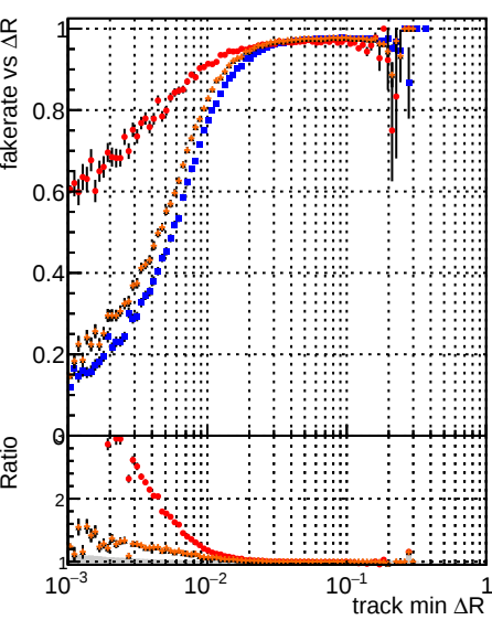
Fake rate vs \Delta R(\text{track, jet}) Line Style Color Series Solid Blue DOM Solid Red CKE Solid Orange TTbar Solid Black TTbar Dashed Blue DOM Dashed Red CKE Dashed Orange TTbar Dashed Black TTbar Dotted Blue DOM Dotted Red CKE Dotted Orange TTbar Dotted Black TTbar Long Dash Blue DOM Long Dash Red CKE Long Dash Orange TTbar Long Dash Black TTbar Short Dash Blue DOM Short Dash Red CKE Short Dash Orange TTbar Short Dash Black TTbar Thin Solid Blue DOM Thin Solid Red CKE Thin Solid Orange TTbar Thin Solid Black TTbar Thin Dashed Blue DOM Thin Dashed Red CKE Thin Dashed Orange TTbar Thin Dashed Black TTbar Thin Dotted Blue DOM Thin Dotted Red CKE Thin Dotted Orange TTbar Thin Dotted Black TTbar Thin Long Dash Blue DOM Thin Long Dash Red CKE Thin Long Dash Orange TTbar Thin Long Dash Black TTbar Thin Short Dash Blue DOM Thin Short Dash Red CKE Thin Short Dash Orange TTbar Thin Short Dash Black TTbar
