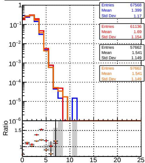
mean hit DQM_CKF_TTbar DQM_mkFit_TTbar DQM_mkFit_TTbarPU-ncp DQM_mkFit_TTbarPU-newTr4
