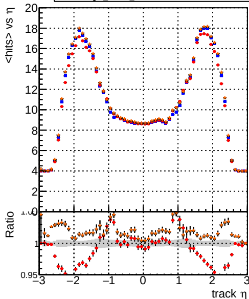
mean hits DQM_CKF_TTbar DQM_mkFit_TTbar DQM_mkFit_TTbarPU-ncp DQM_mkFit_TTbarPU-newTr4
