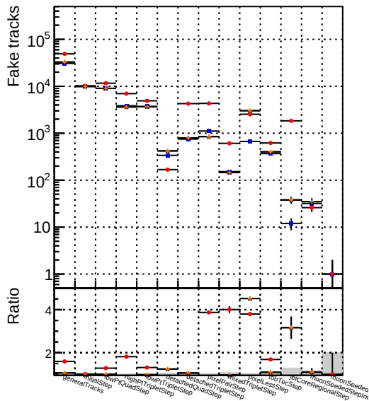
Number of tracks vs collection Legend: DQM_CKF_TTbar DQM_mkFit_TTbar DQM_mkFit_TTbarPU-ncp DQM_mkFit_TTbarPU-newTr4
