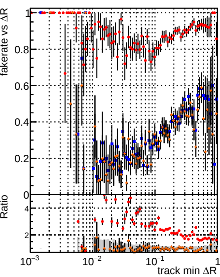
Fake rate vs \Delta R (track, jet) for various models and methods. Legend: DOM (black), CKF (blue), TTbar (red), mktFit (orange), PU-ncp (grey), PU-newTr4 (light blue).
