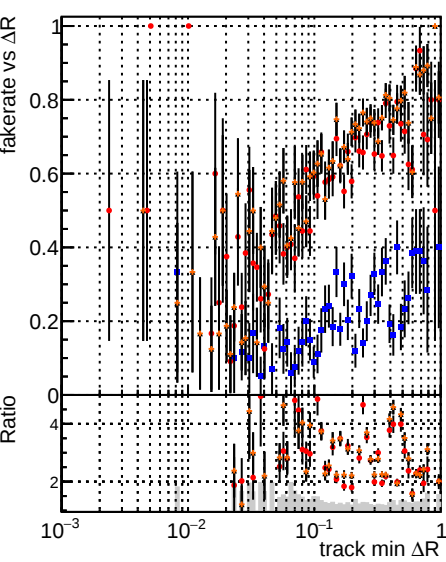
Fake rate vs \Delta R(\text{track, jet}) DOM CKF TTbar DOM mktFit TTbar DOM mktFit TTbar PU-ncp DOM mktFit TTbar PU-newTr4
