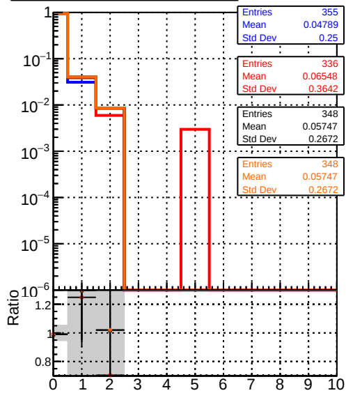
DQM_CKF_TTbar DQM_mkFit_TTbar DQM_mkFit_TTbarPU-ncp DQM_mkFit_TTbarPU-newTr4 mean hit
