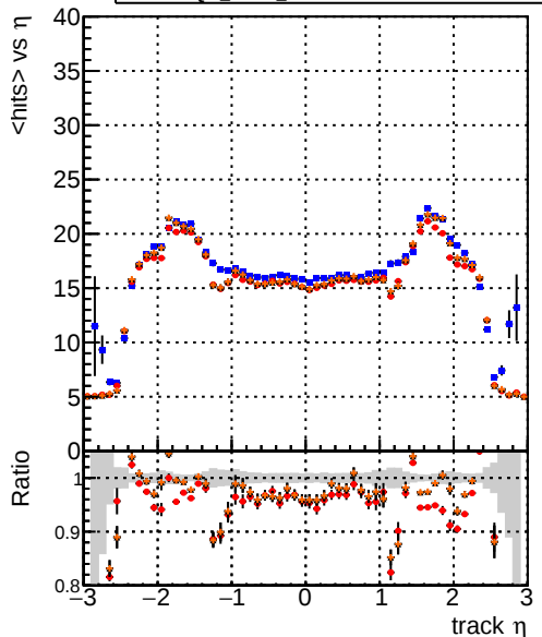
mean hit — DQM_CKF_TTbar — DQM_mkFit_TTbar — DQM_mkFit_TTbarPU-ncp — DQM_mkFit_TTbarPU-newTr4
