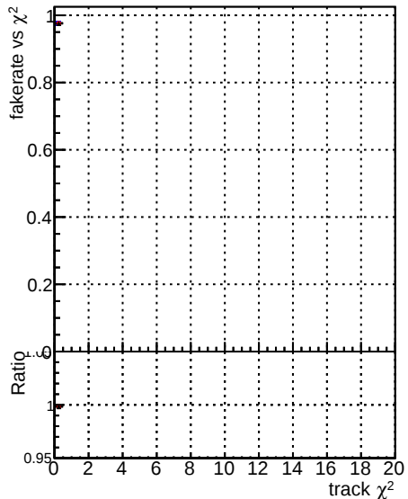
Fake rate vs. DOM CKF TTbar DOM mktFit TTbarPU-nep DOM mktFit TTbarPU-newTr4
