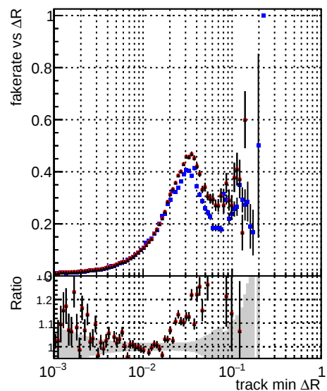
Legend for Fake rate vs \Delta R , Duplicates Rate vs \Delta R , and Pileup rate vs \Delta R : \blacksquare DOM_CKF_TTbar \bullet DOM_mkFit_TTbarPU-ncp \times DOM_mkFit_TTbarPU-newTr4
