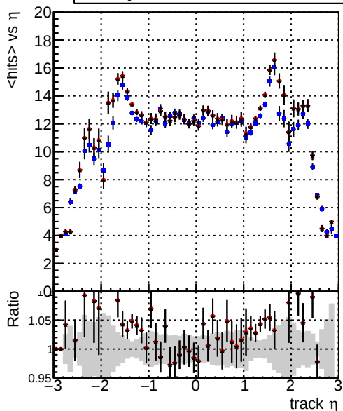
mean hits — DQM_CKF_TTbar — DQM_mkFit_TTbarPU-ncp — DQM_mkFit_TTbarPU-newTr4
