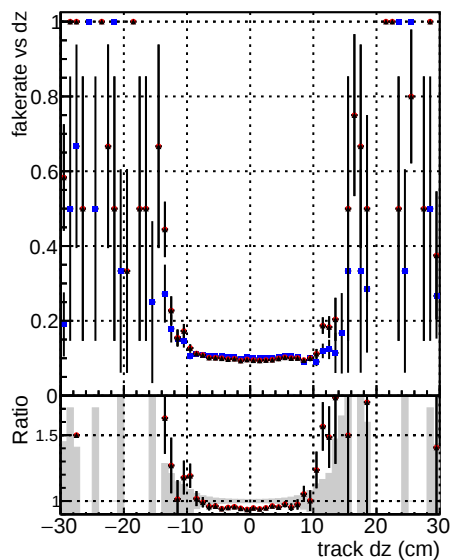
DOM CKF T\bar{T} bar PU-ncp DOM mktFit T\bar{T} bar PU-newTr4
