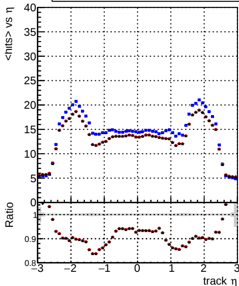
mean hit — DQM_CKF_TTbar — DQM_mkFit_TTbarPU-ncp — DQM_mkFit_TTbarPU-newTr4
