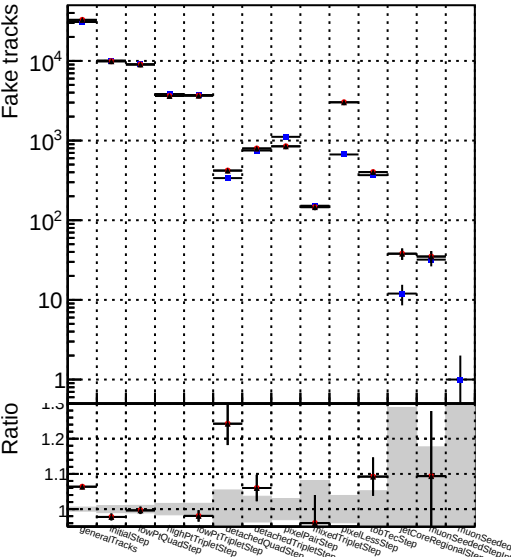
Number DQM_mkFit_TTbarPU-ncp DQM_mkFit_TTbarPU-newTr4
