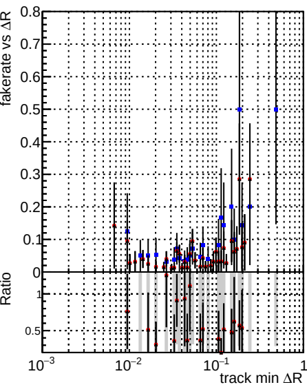
Fake rate vs \Delta R(\text{track}, \text{jet}) DQM_CKF_TTbar DQM_mkFit_TTbarPU-ncp DQM_mkFit_TTbarPU-newTr4
