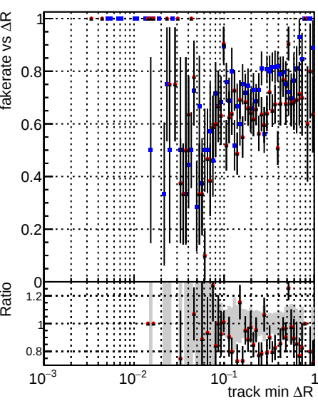
Fake rate vs \Delta R(\text{track, jet}) DOM_CKF_TTbar DOM_mkFit_TTbarPU-ncp DOM_mkFit_TTbarPU-newTr4
