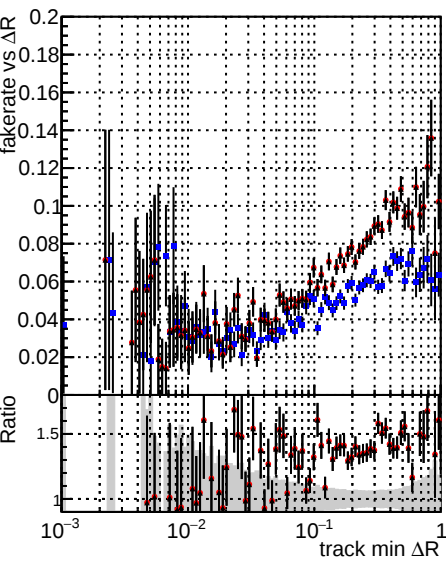
Legend: DQM_CKF_TTbar (blue circles), DQM_mkFit_TTbarPU-ncp (red circles), DQM_mkFit_TTbarPU-newTr4 (black circles)
