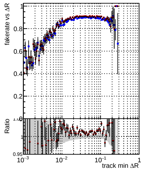
—•— DQM_CKF_TTbar —•— DQM_mkFit_TTbarPU-ncp —•— DQM_mkFit_TTbarPU-newTr4
