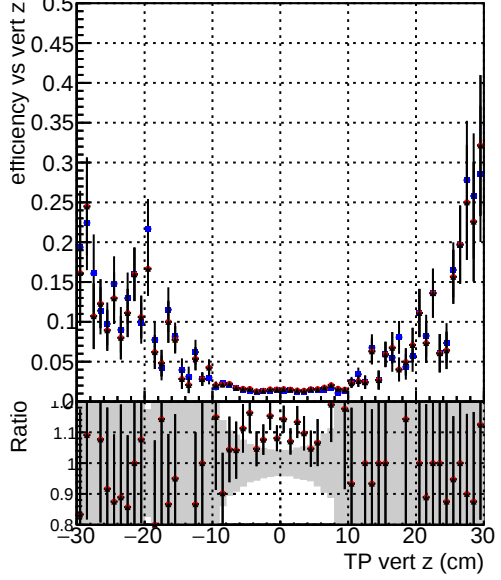
Efficiency vs. TP vert z (cm) — DQM_CKF_TTbar — DQM_mkFit_TTbarPU-ncp — DQM_mkFit_TTbarPU-newTr4
