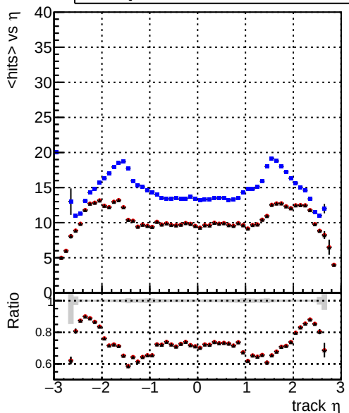
mean hit — DQM_CKF_TTbar — DQM_mkFit_TTbarPU-ncp — DQM_mkFit_TTbarPU-newTr4
