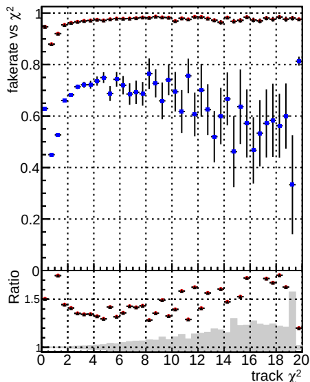
Fake rate vs. DOM CKF T\bar{T} bar DOM mktFit T\bar{T} barPU-hcp DOM mktFit T\bar{T} barPU-hewTr4
