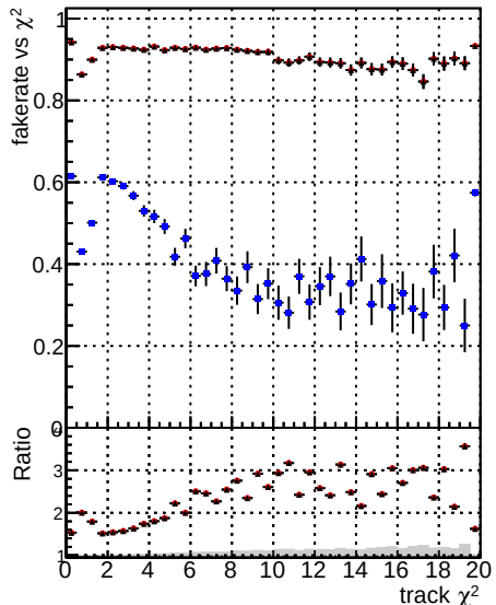
Fake rate vs. DOM CKF TTbar DOM mktFit TTbarPU-ncp DOM mktFit TTbarPU-newTr4
