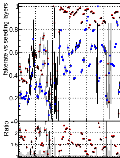
Fake rate vs. DOM CKF TTbar DOM mktFit TTbarPU-ncp DOM mktFit TTbarPU-newTr4
