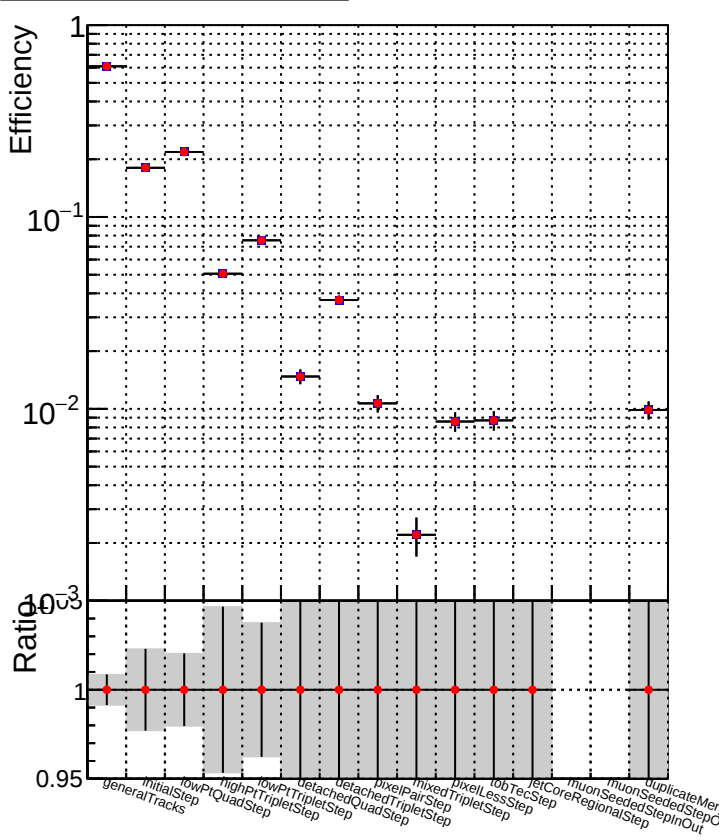
DQM_V0001_R000000001_Global_CMSSW_NOBATCH_RECO DQM_V0001_R000000001_Global_CMSSW_BATCH_RECO
