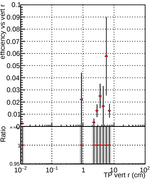
Efficiency vs TP vert r (cm) Legend: DQM_V0001_R0000000001_Global_CMSSW_NOBATCH_RECO DQM_V0001_R0000000001_Global_CMSSW_BATCH_RECO
