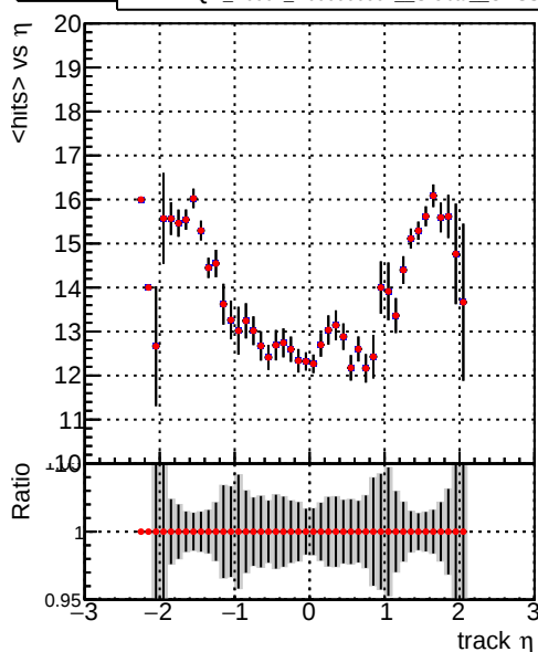
DQM_V0001_R000000001_Global_CMSSW_BATCH_RECO
