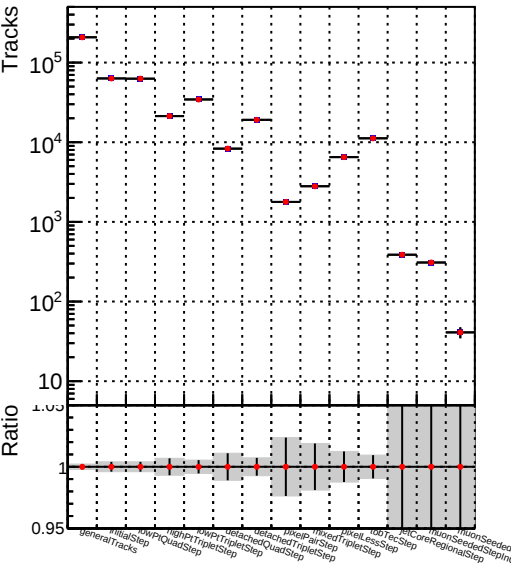
DQM_V0001_R000000001_Global_CMSSW_NOBATCH_RECO
