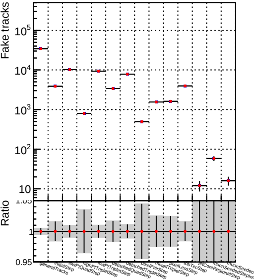
Number —●— DQM_V0001_R000000001 Global CMSSW_BATCH RECO
