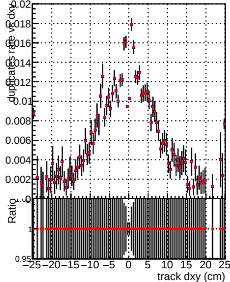
Global CMSSW NOBATCH RECO DQM_V0001_R0000000001 Global CMSSW BATCH DQM_V0001_R0000000001 Global CMSSW BATCH
