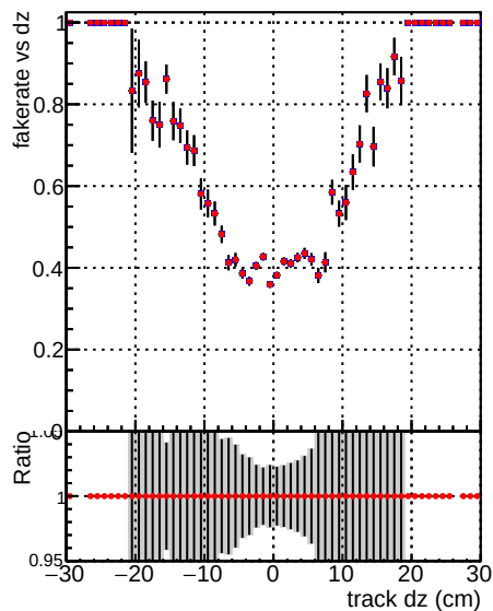
Fake rate vs d —●— DQM V0001_R000000001 Global CMSSW NOBATCH RECO —●— DQM V0001_R000000001 Global CMSSW BATCH RECO
