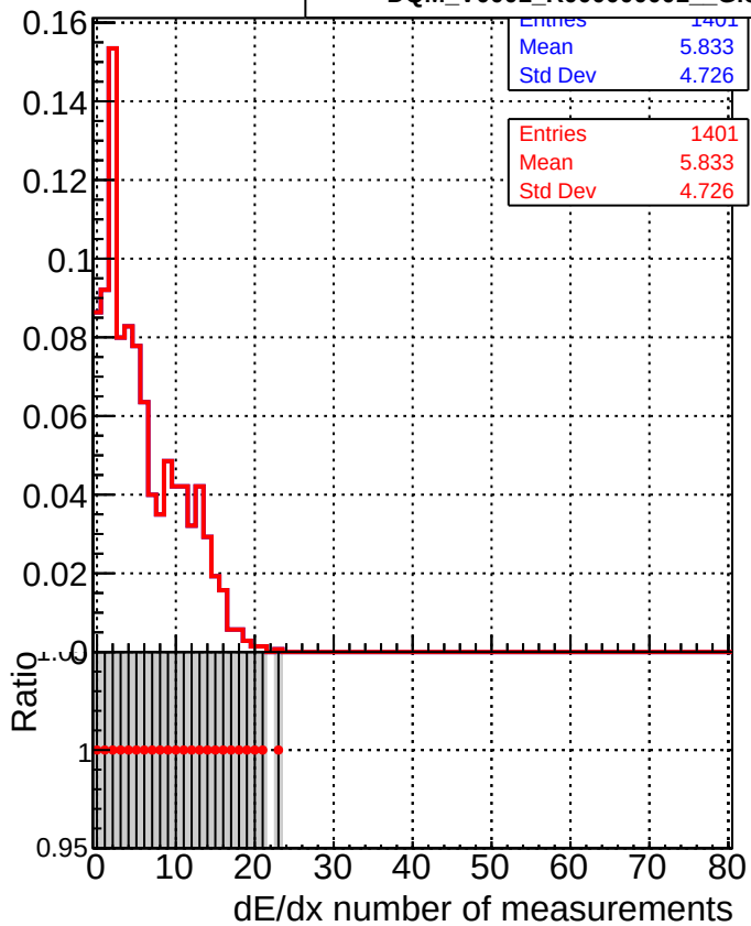
—■— DQM_V0001_R000000001_Global_CMSSW_NOBATCH_RECO —●— DQM_V0001_R000000001_Global_CMSSW_BATCH_RECO
