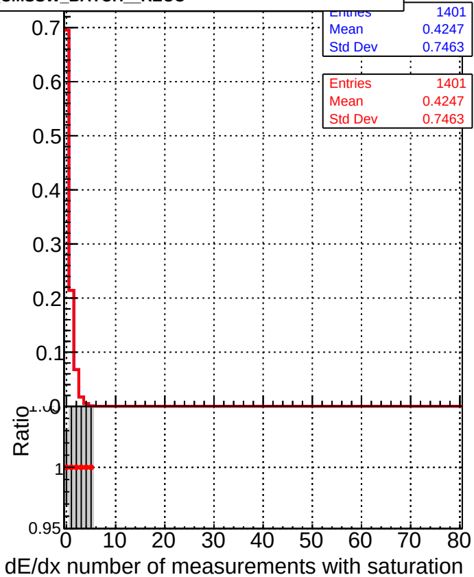
—■— DQM_V0001_R000000001_Global_CMSSW_NOBATCH_RECO —●— DQM_V0001_R000000001_Global_CMSSW_BATCH_RECO
