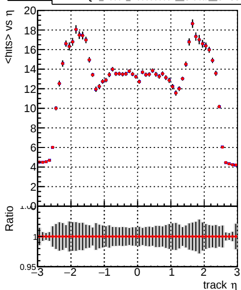
DQM_V0001_R000000001_Global_CMSSW_BATCH_RECO
