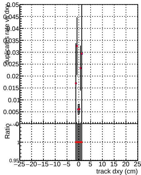
al CMSSW_NOBATCH_RECO al CMSSW_BATCH_RECO
