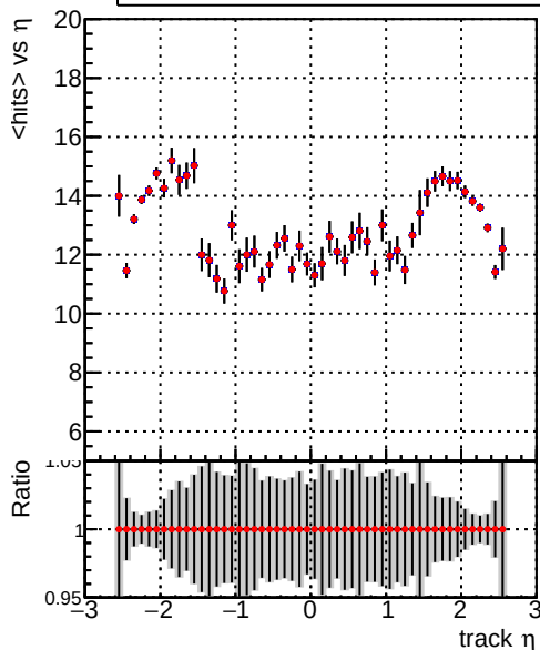
mean hits — DQM_V0001_R000000001_Global_CMSSW_NOBATCH_RECO — DQM_V0001_R000000001_Global_CMSSW_BATCH_RECO
