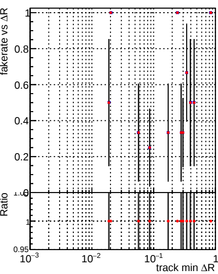
Legend: DQM_V0001_R000000001_Global_CMSSW_NOBATCH_RECO DQM_V0001_R000000001_Global_CMSSW_BATCH_RECO
