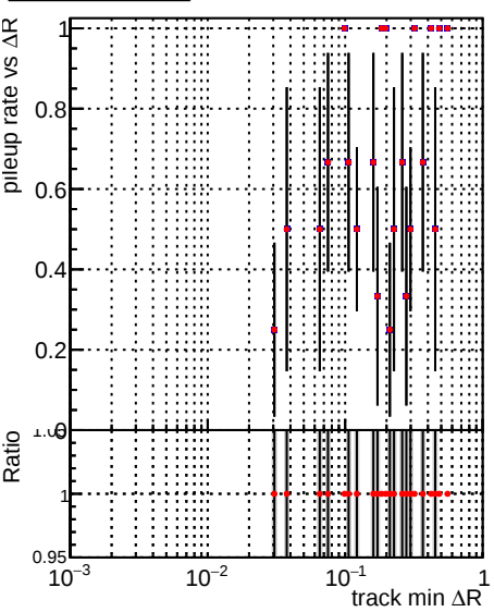
Legend: DQM_V0001_R000000001_Global_CMSSW_NOBATCH_RECO DQM_V0001_R000000001_Global_CMSSW_BATCH_RECO
