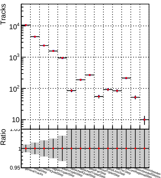
DQM_V0001_R000000001__Global__CMSSW_NOBATCH__RECO
