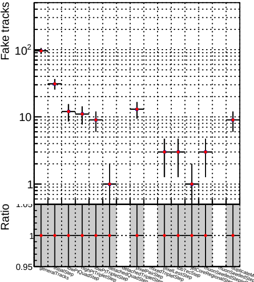
Number —• DOM V0001 R000000001 Global CMSSW BATCH RECO
