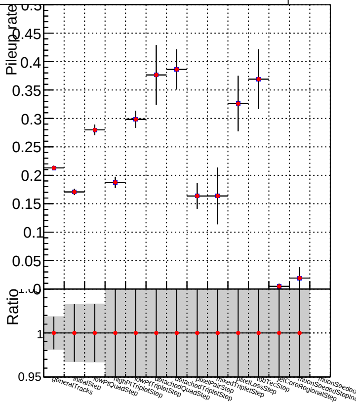
DQM_V0001_R000000001_Global_CMSSW_NOBATCH_RECO DQM_V0001_R000000001_Global_CMSSW_BATCH_RECO
