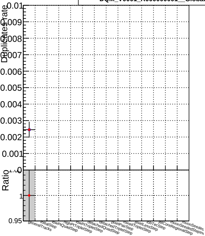
DQM_V0001_R000000001_Global_CMSSW_NOBATCH_RECO DQM_V0001_R000000001_Global_CMSSW_BATCH_RECO
