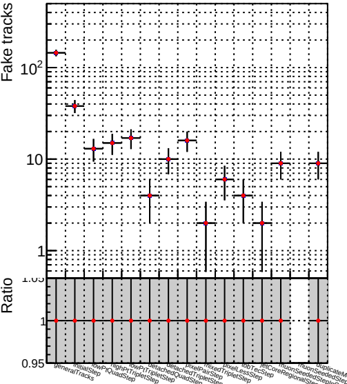
Number ● DQM_V0001 R000000001 Global CMSSW_BATCH RECO
