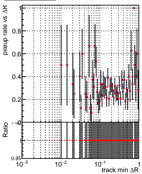
█ DQM_V0001_R000000001_Global_CMSSW_NOBATCH_RECO █ DQM_V0001_R000000001_Global_CMSSW_BATCH_RECO
