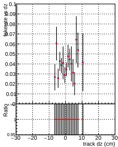
Fake rate vs dz —●— DQM_V0001_R0000000001_Global_CMSSW_NOBATCH_RECO —●— DQM_V0001_R0000000001_Global_CMSSW_BATCH_RECO
