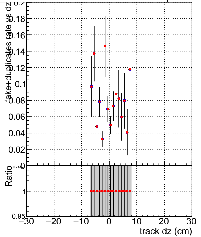
DQM_V0001_R000000001_Global_CMSSW_NOBATCH_RECO DQM_V0001_R000000001_Global_CMSSW_BATCH_RECO
