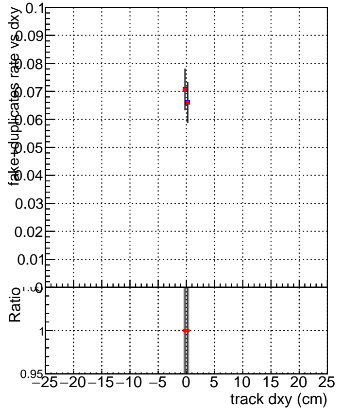
DQM_V0001_R000000001_Global_CMSSW_NOBATCH_RECO DQM_V0001_R000000001_Global_CMSSW_BATCH_RECO
