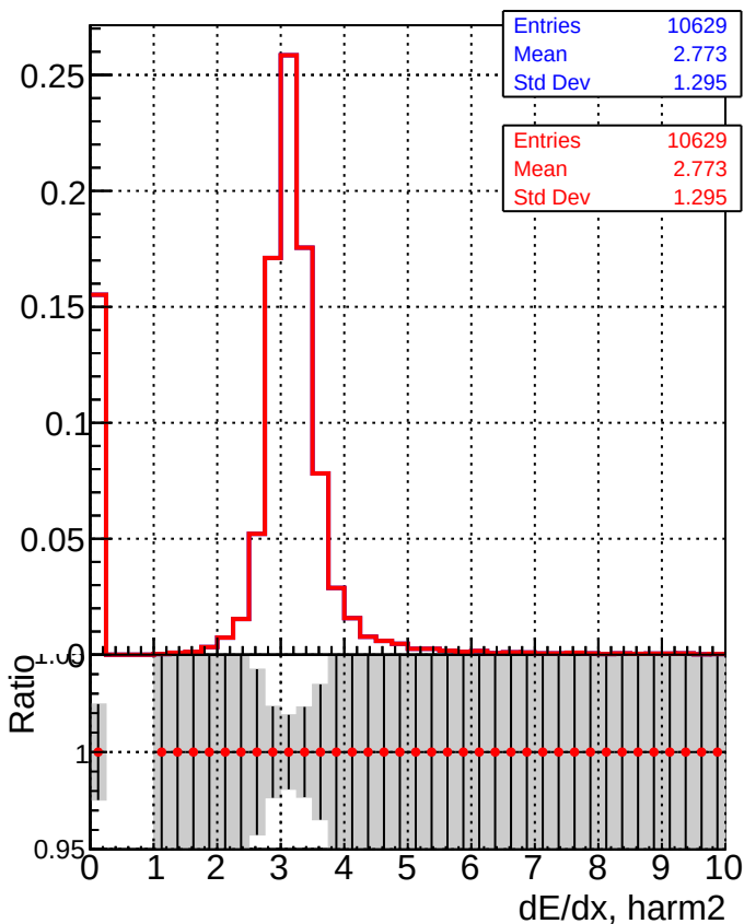
DQM_V0001_R000000001_Global_CMSSW_NOBATCH_RECO DQM_V0001_R000000001_Global_CMSSW_BATCH_RECO
