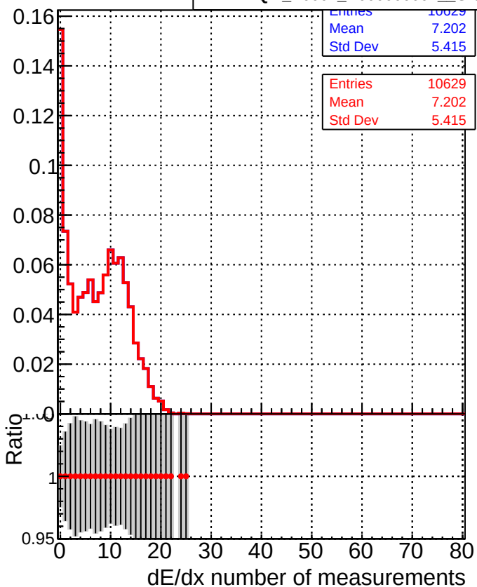
DQM_V0001_R000000001_Global_CMSSW_NOBATCH_RECO DQM_V0001_R000000001_Global_CMSSW_BATCH_RECO
