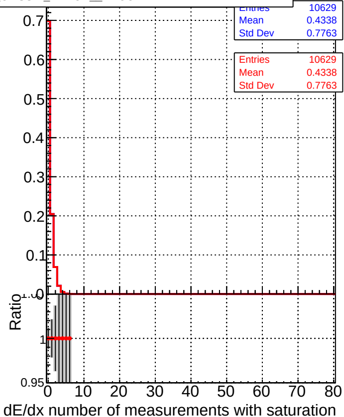
DQM_V0001_R000000001_Global_CMSSW_NOBATCH_RECO DQM_V0001_R000000001_Global_CMSSW_BATCH_RECO
