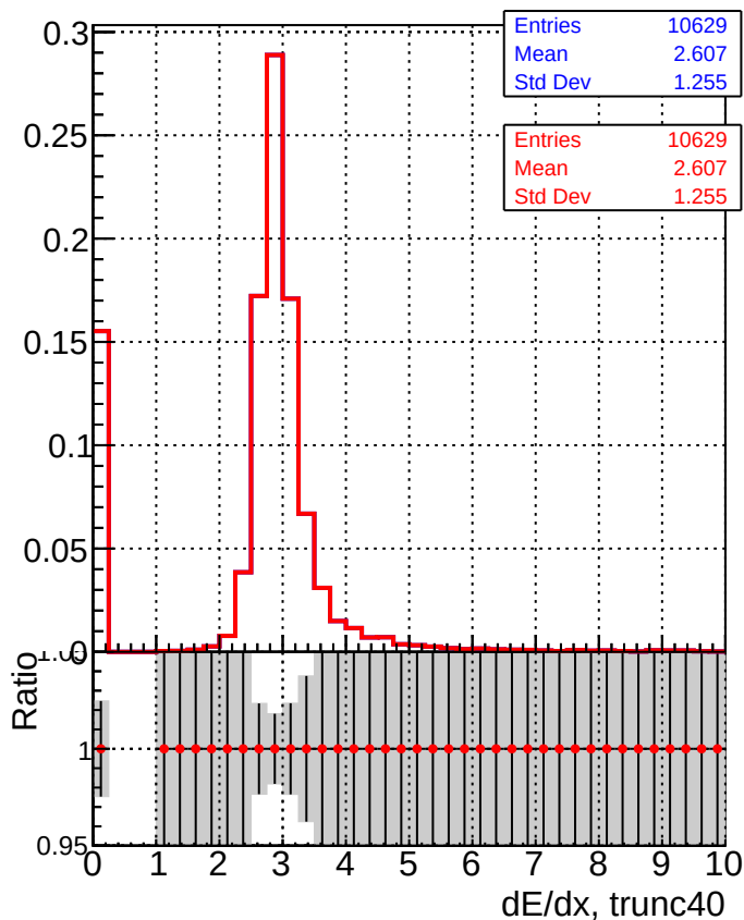
DQM_V0001_R000000001_Global_CMSSW_NOBATCH_RECO DQM_V0001_R000000001_Global_CMSSW_BATCH_RECO
