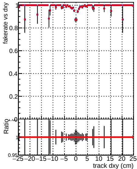
DQM_V0001_R0000000001 Global CMSSW_NOBATCH_RECO Fake rate vs d DQM_V0001_R0000000001 Global CMSSW_BATCH_RECO
