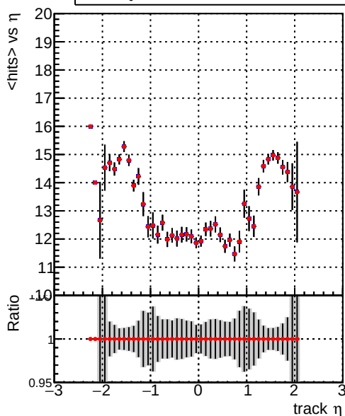
— DQM_V0001_R000000001_Global_CMSSW_NOBATCH_RECO — DQM_V0001_R000000001_Global_CMSSW_BATCH_RECO
