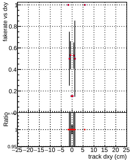
—●— DQM_V0001_R0000000001_Global_CMSSW_NOBATCH_RECO —●— DQM_V0001_R0000000001_Global_CMSSW_BATCH_RECO
