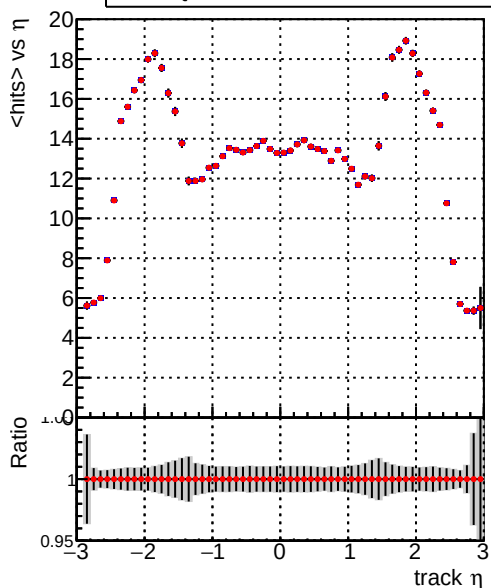
DQM_V0001_R000000001_Global_CMSSW_BATCH_RECO
