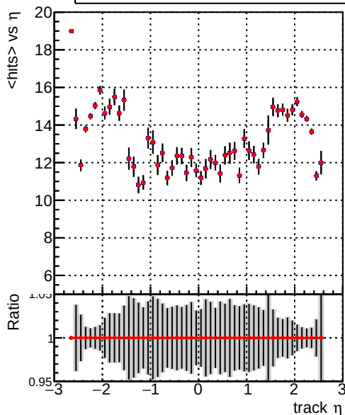
mean hit — DQM_V0001_R000000001_Global_CMSSW_NOBATCH_RECO — DQM_V0001_R000000001_Global_CMSSW_BATCH_RECO
